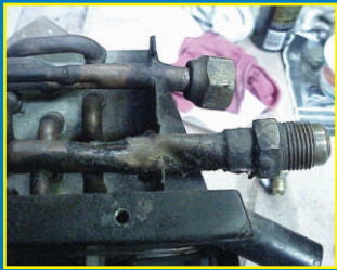
AC COILS
